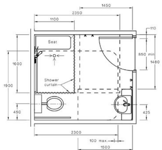
FIGURE 51(b) SANITARY COMPARTMENT SHOWING OVERLAP OF WASHBASIN FIXTURE INTO SHOWER CIRCULATION SPACE
