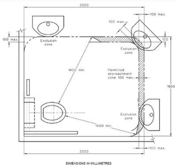
FIGURE 51(a) SANITARY COMPARTMENT SHOWING OVERLAP OF WASHBASIN FIXTURE INTO CIRCULATION SPACE FOR WATER CLOSET
